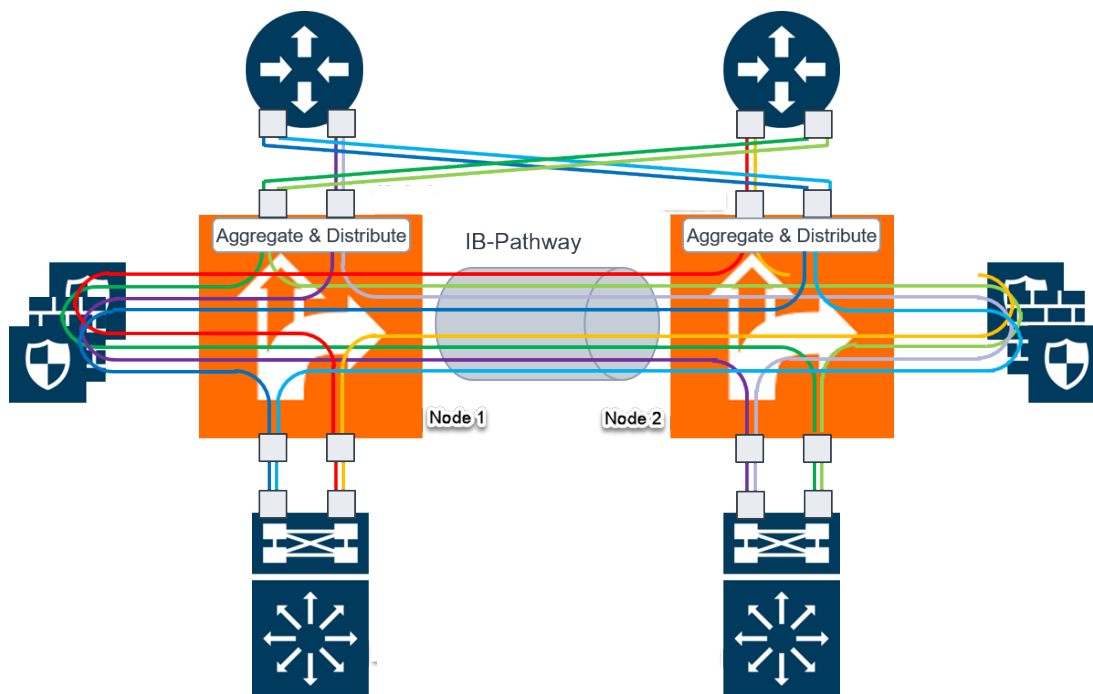
Figure 52 Resilient Inline Arrangement
