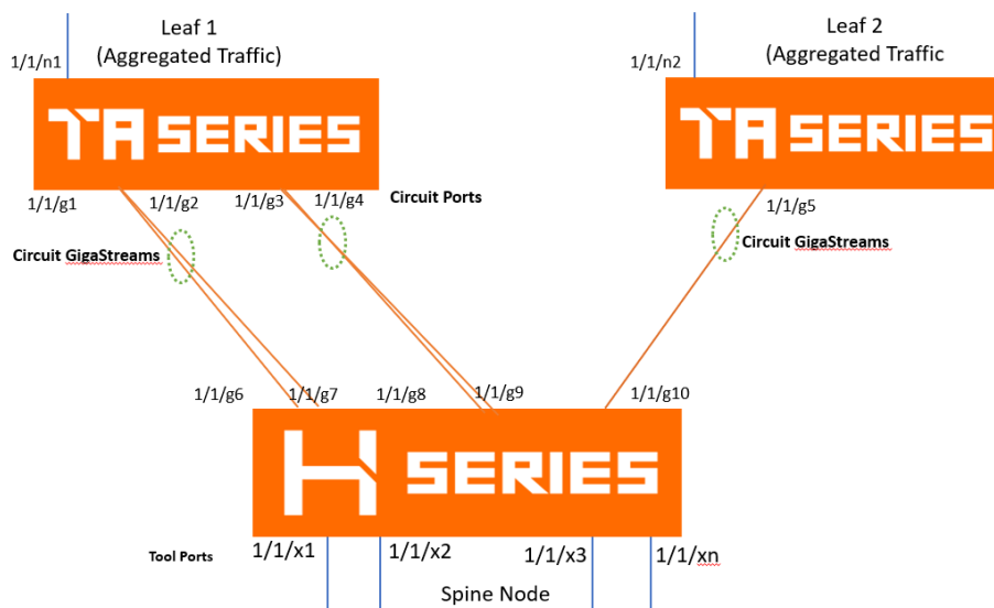
Figure 66 Circuit GigaStreams in Fabric Maps
