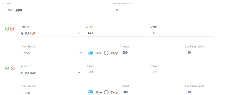
Figure 89 Advanced Flow Slicing
