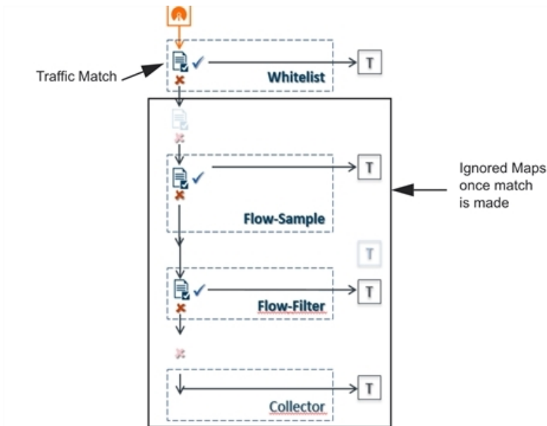
Figure 39 Non-Overlap GTP Mapping Mode
